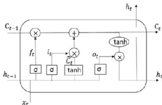
Figure 5. LSTM Model
