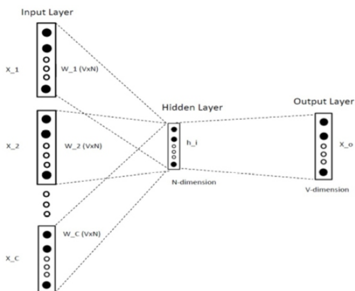
Figure 1. CBOW Model
