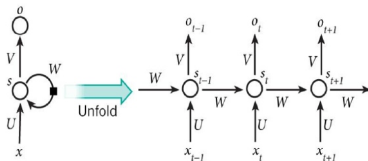
Figure 4. RNN Model
